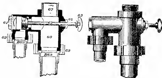
Fig. 1682. Section.
